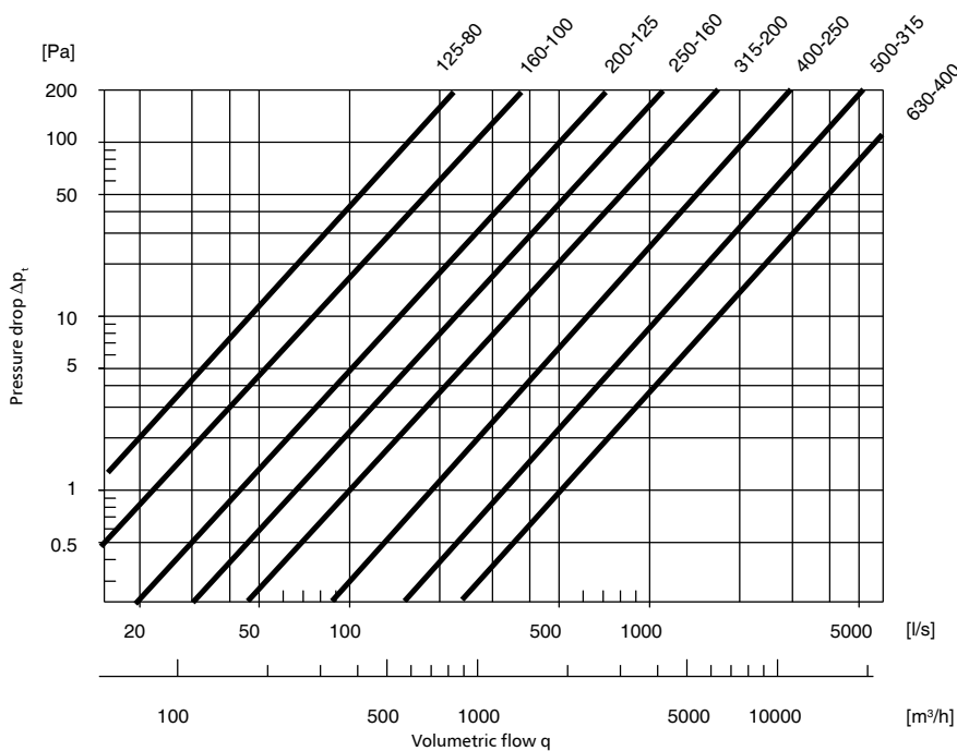
2 reduction stage
